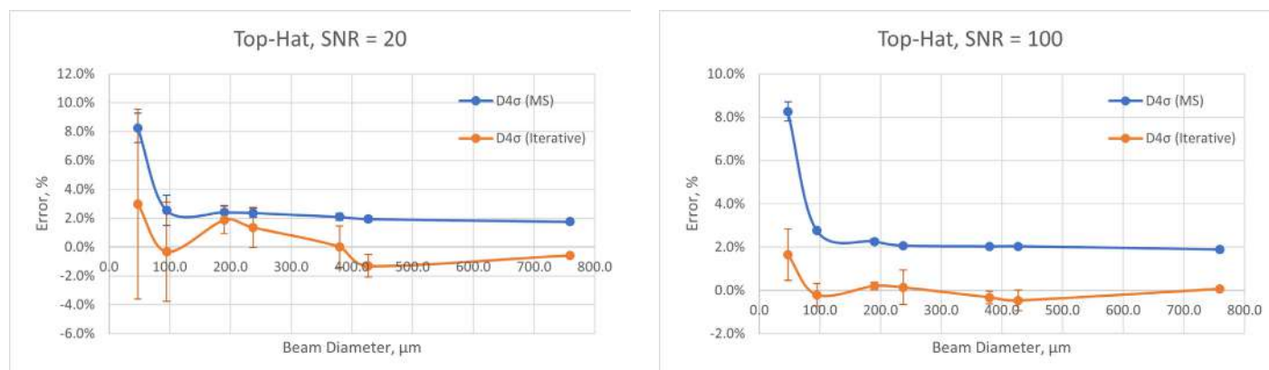
Figure 4 - Error of Beam Width Measurement as a Function of Beam Width for Top-Hat Beams
