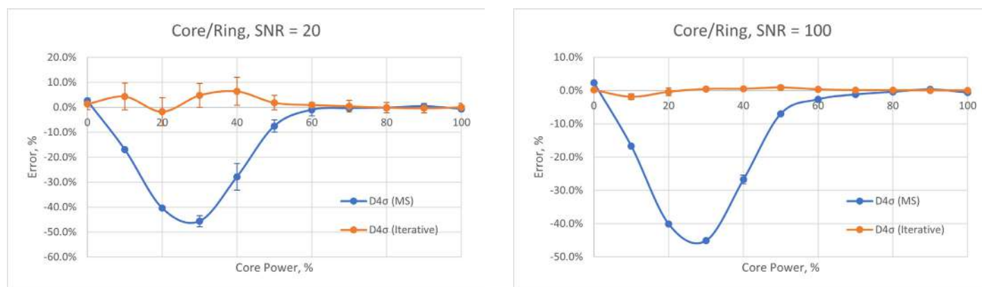
Figure 6 - Error of Beam Width Measurement as a Function of Core Power
