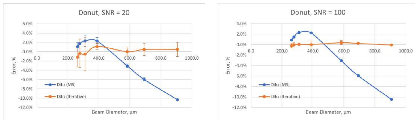
Figure 5 - Error of Beam Width Measurement as a Function of Beam Width for Donut Beams
