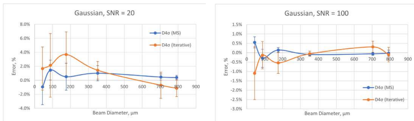
Figure 3 - Error of Beam Width Measurement as a Function of Beam Width for Gaussian Beams
